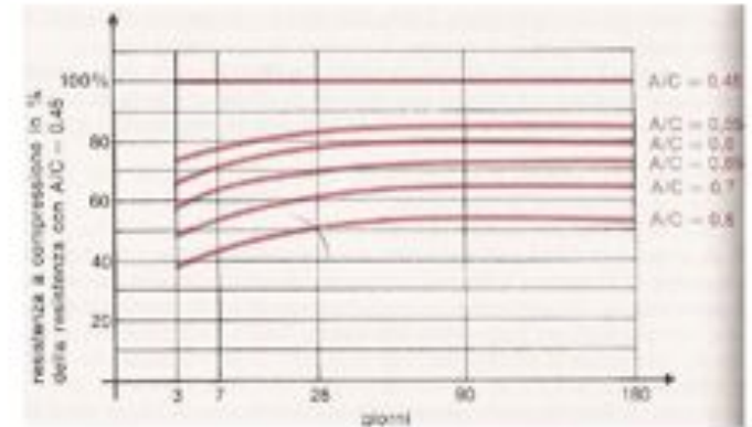
Variation of concrete strength at different water-cement ratios
